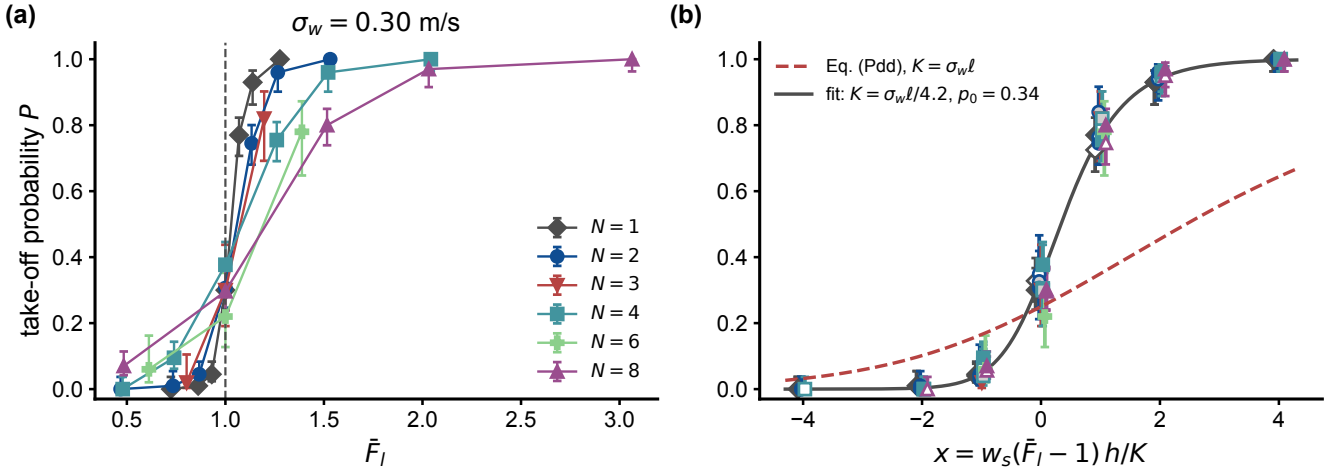
FIG. 7. Take-off probability in synthetic turbulence ( \ell = 1 m, U_h = 1 m/s, z_0 = 0.5 m, h = 2 m, tip charge, m = 1 mg, Q_s = 0 , N_t = 50 ). Markers: ensemble estimates from Algorithm 2 with 95% Wilson intervals ( M = 200 for |x| \leq 1 , M = 100 otherwise; M = 50 for N = 3, 6 and \sigma_w = 0.22 m/s). (a) P versus \bar{F}_l for \sigma_w = 0.30 m/s; the vertical dashed line marks the deterministic threshold \bar{F}_l = 1 . (b) All valid grid points versus the scaled drift x = w_s(\bar{F}_l - 1)h/K , K = \sigma_w\ell ; open markers \sigma_w = 0.15 , grey 0.22, filled 0.30 m/s, small horizontal offsets for readability. Dashed: Eq. (18) with K = \sigma_w\ell ; solid: Eq. (18) with K_{\text{eff}} = \sigma_w\ell/a and start fraction p_0 fitted to all points ( a = 4.2 , p_0 = 0.34 ).
