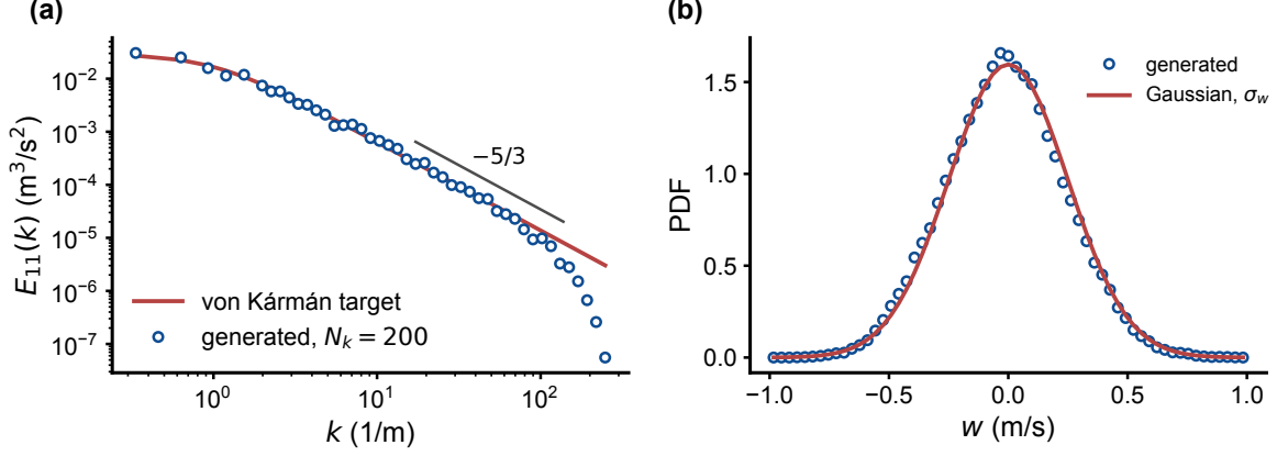
FIG. 6. Validation of the synthetic turbulence of Eq. (15), for \sigma_w = 0.25 m/s, \ell = 1 m, and N_k = 200 modes (average over 50 realizations). (a) Longitudinal one-dimensional spectrum of w along a vertical line versus the spectrum implied by Eq. (16); the generated spectrum is shown up to the cut-off k_{\max} = 2\pi/(5 \times 5 \text{ mm}) = 251 \text{ m}^{-1} and falls below the target above k \approx 80 \text{ m}^{-1} because of the finite shell width near k_{\max} . (b) Probability density of w with the Gaussian of standard deviation \sigma_w ; the sample standard deviation is 0.249 m/s. Mode amplitudes renormalized as in Appendix D.
