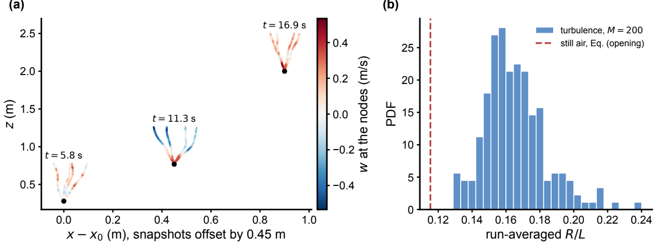
FIG. 8. Deformation of the bundle by turbulence ( N = 4 , q = 0.331 nC, \bar{F}_l = 1 , \sigma_w = 0.30 m/s, \ell = 1 m). (a) One rising realization at three instants, side view in the frame of the spider (panels offset horizontally); nodes coloured by the vertical air velocity w at the node. (b) Distribution over the M = 200 realizations of the time-averaged tip radius R/L , compared with the still-air value of Eq. (31) at \bar{F}_l = 1 ( \tau = 1 , g = 1 ).
